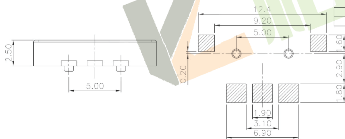
P.C.B Mounting Pattern Dimension
