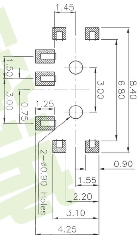
PCB Layout (Pattern side)
