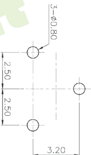
HOLE LAYOUT
