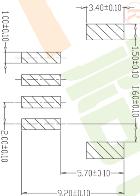
PCB LAYOUT
