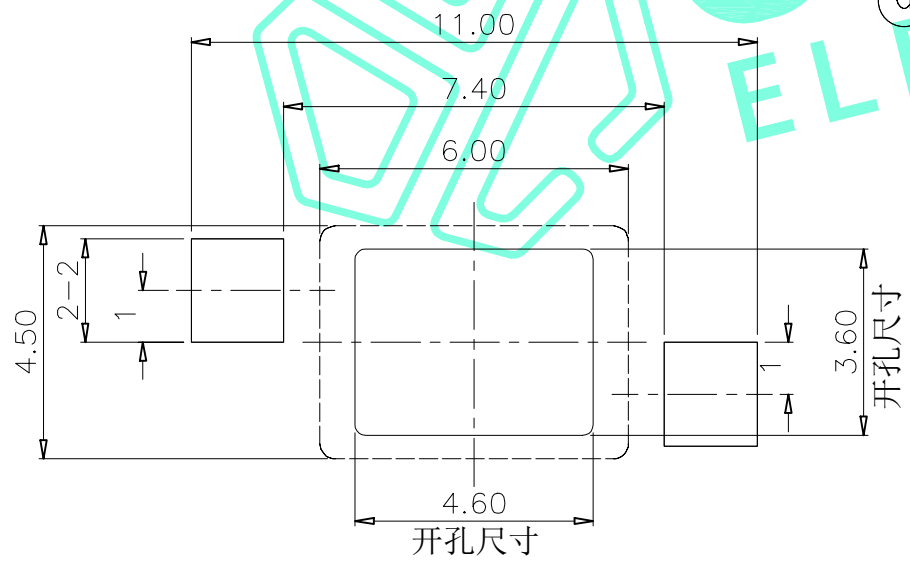
Hole Layout(top view)
