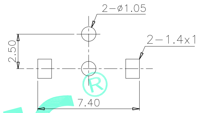
HOLE LAYOUT
