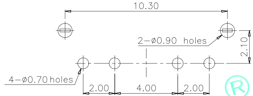
PCB Layout (Pattern side)
