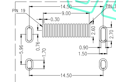
RECOMMENDED P.C.B HOLE LAYOUT COMPONENT SIDE VIEW(TOLERANCE: +/-0.05)
