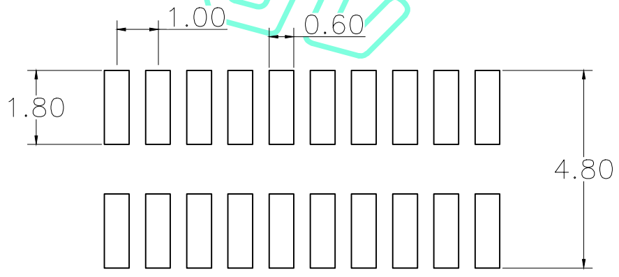
Recommended P.C.B Hloe Layout
