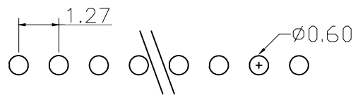
Recommended P.C.B Hloe Layout
