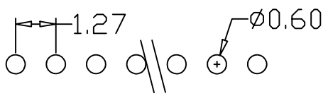
Recommended P.C.B Hlow Layout
