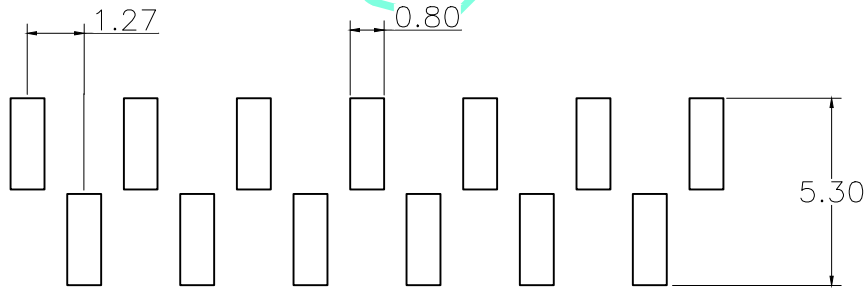
Recommended P.C.B Hlow Layout
