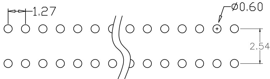
Recommended P.C.B Hlow Layout
