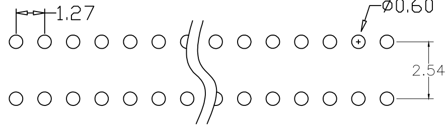
Recommended P.C.B Hloe Layout
