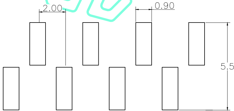
Recommended P.C.B Hlow Layout
