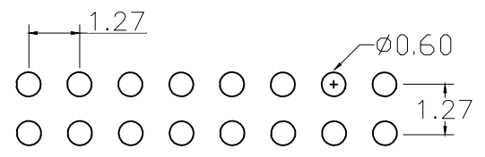
Recommended P.C.B Hloe Layout
