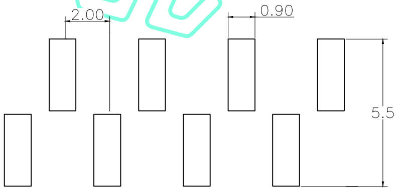
Recommended P.C.B Hlow Layout
