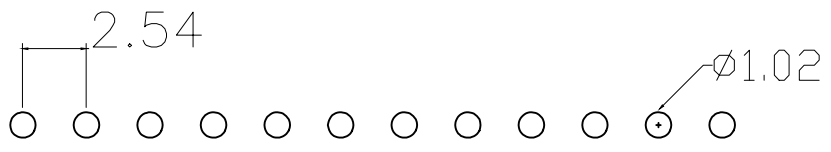
Recommended P.C.B Hloe Layout
