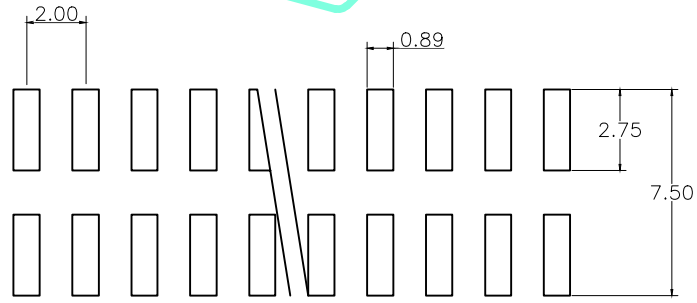
Recommended P.C.B Hloe Layout
