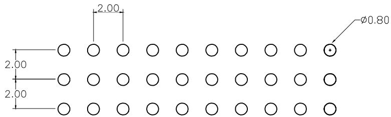
Recommended P.C.B Hloe Layout
