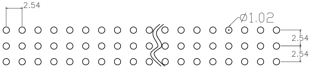
Recommended P.C.B Hlow Layout
