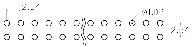
Recommended P.C.B Hlow Layout
