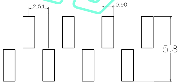
Recommended P.C.B Hloe Layout
