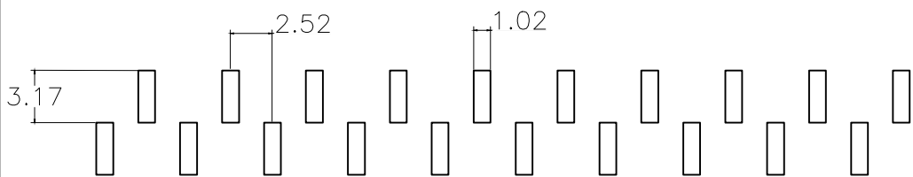
Recommended P.C.B Hloe Layout TYPE-2
