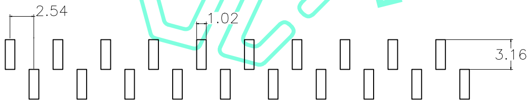
Recommended P.C.B Hloe Layout TYPE-1
