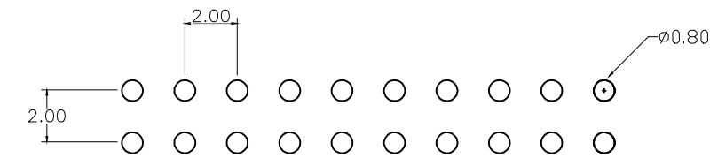
Recommended P.C.B Hlow Layout
