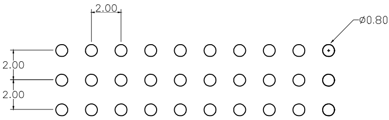
Recommended P.C.B Hlow Layout
