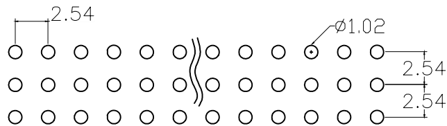
Recommended P.C.B Hlow Layout
