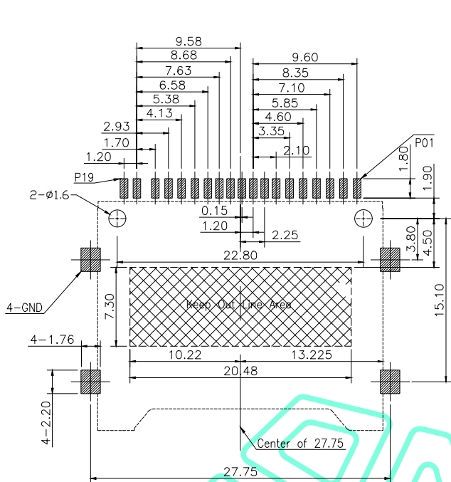
Recommended PCB Layout Tolerance : ± 0.05
